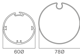
RULLO - TUBE
